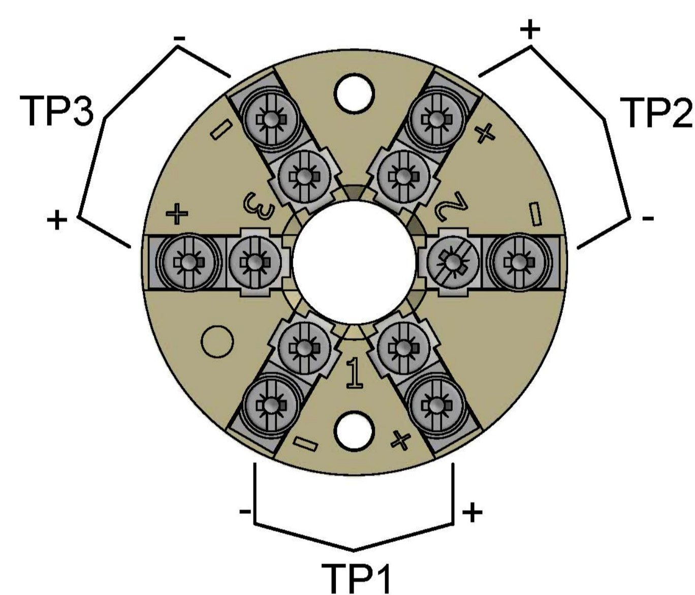
Terminal base model A 3 thermocouples
