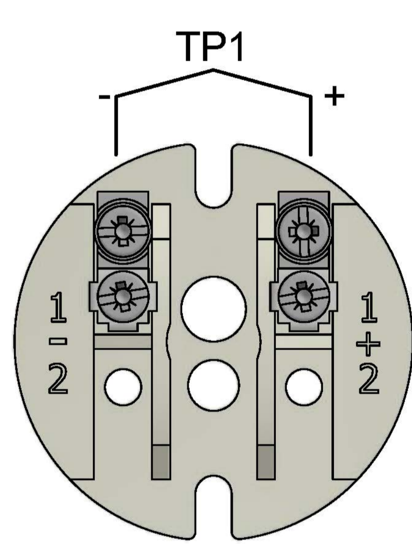
Terminal base model A with separate test hole
